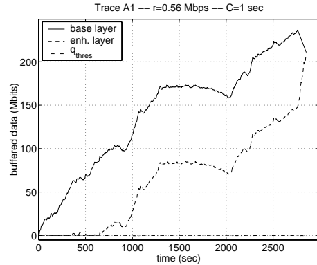
Fig. 7. Buffered data for dynamic threshold policies with C = C' = 1 second.
